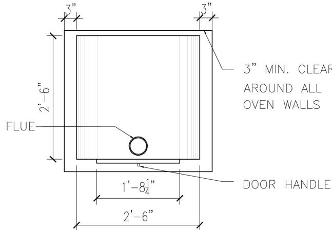
1 PLAN 1/2" = 1'-0"
