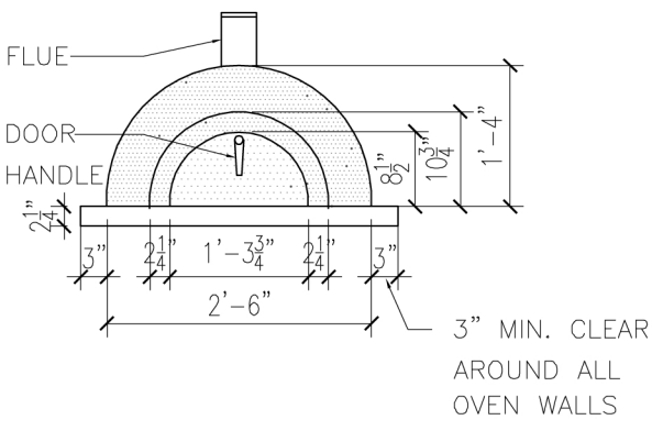
2 FRONT ELEVATION 1/2" = 1'-0"
