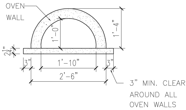
4 SECTION 1/2" = 1'-0"
