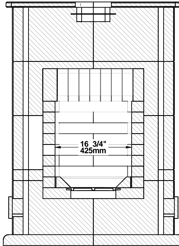
SECTION B-B
